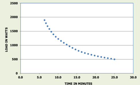
2503 LFP BATTERY RUN TIME VERSUS POWER (ROOM TEMPERATURE TESTING CONDITIONS)
