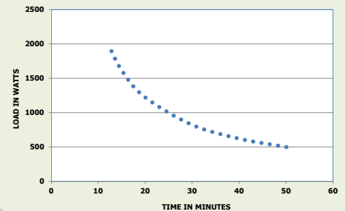
LFP 2500 BATTERY RUN TIME VERSUS POWER (ROOM TEMPERATURE TESTING CONDITIONS)
