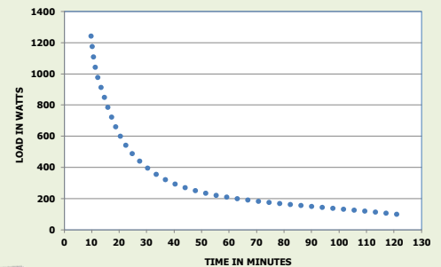
LFP 1252 BATTERY RUN TIME VERSUS POWER (ROOM TEMPERATURE TESTING CONDITIONS)
