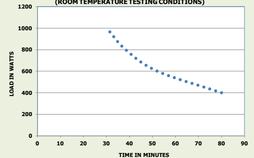
LFP 1251 C1 BATTERY RUN TIME VERSUS LOAD UPS internal battery plus C1 two external batteries (ROOM TEMPERATURE TESTING CONDITIONS)
