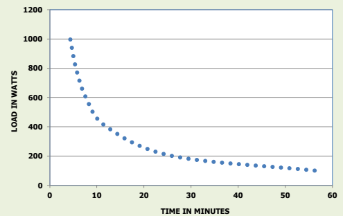
VRLA 1252 BATTERY RUN TIME VERSUS POWER (ROOM TEMPERATURE TESTING CONDITIONS)
